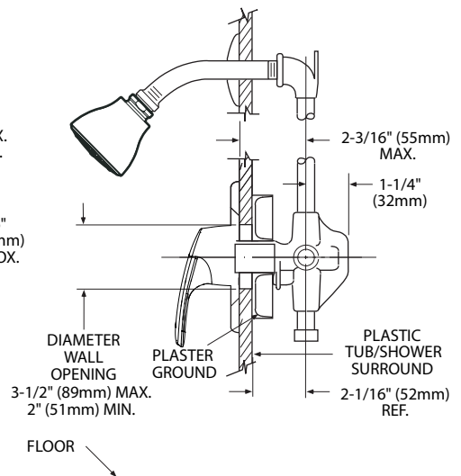
THIN WALL APPLICATION
