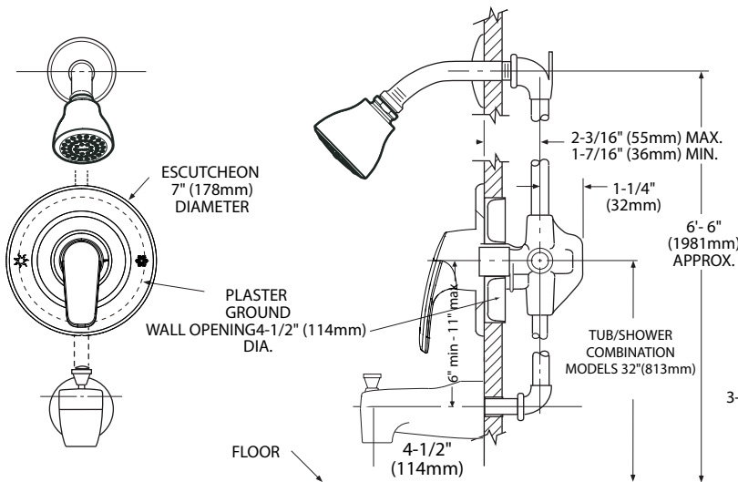
THICK WALL APPLICATION
