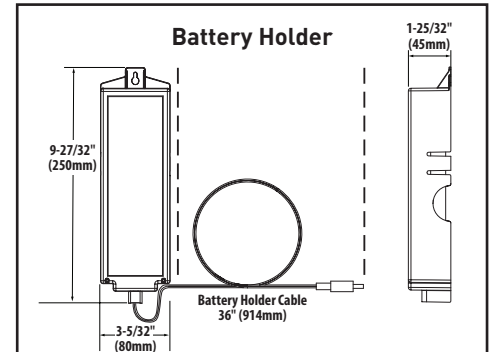
CRITICAL DIMENSIONS DO NOT SCALE
