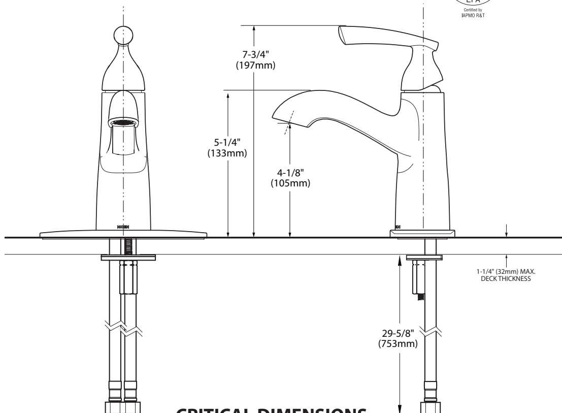
CRITICAL DIMENSIONS (DO NOT SCALE)
