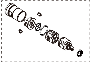
Cartridge Assembly 1213
